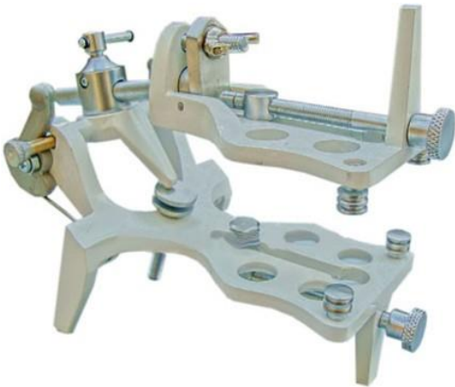
PLASTERLESS ARTICULATOR GALETTI (WHITE) PS-81-101
