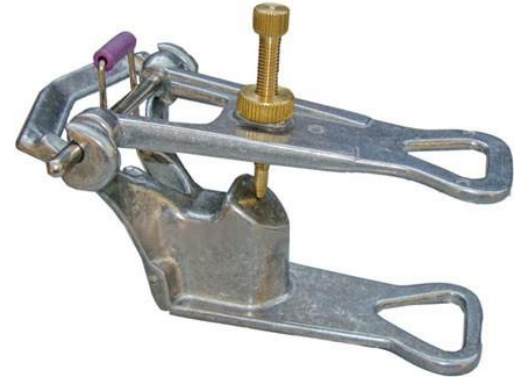
PROFESSIONAL OCCLUSOR ARTICULATOR PS-81-109
